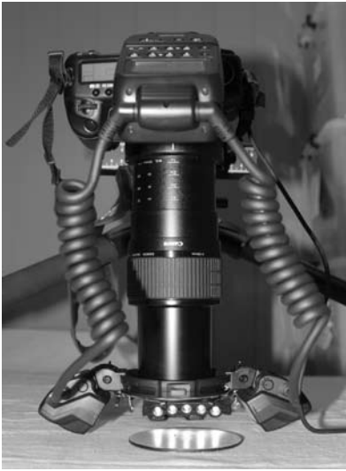
Figure 6. Front view of set-up above sample plate.
